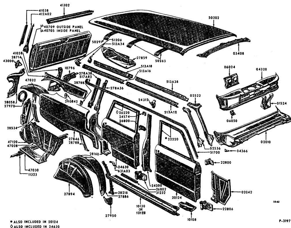
1960-61 FALCON STATION WAGON UPPER BODY - BODY TYPE X (71A)
