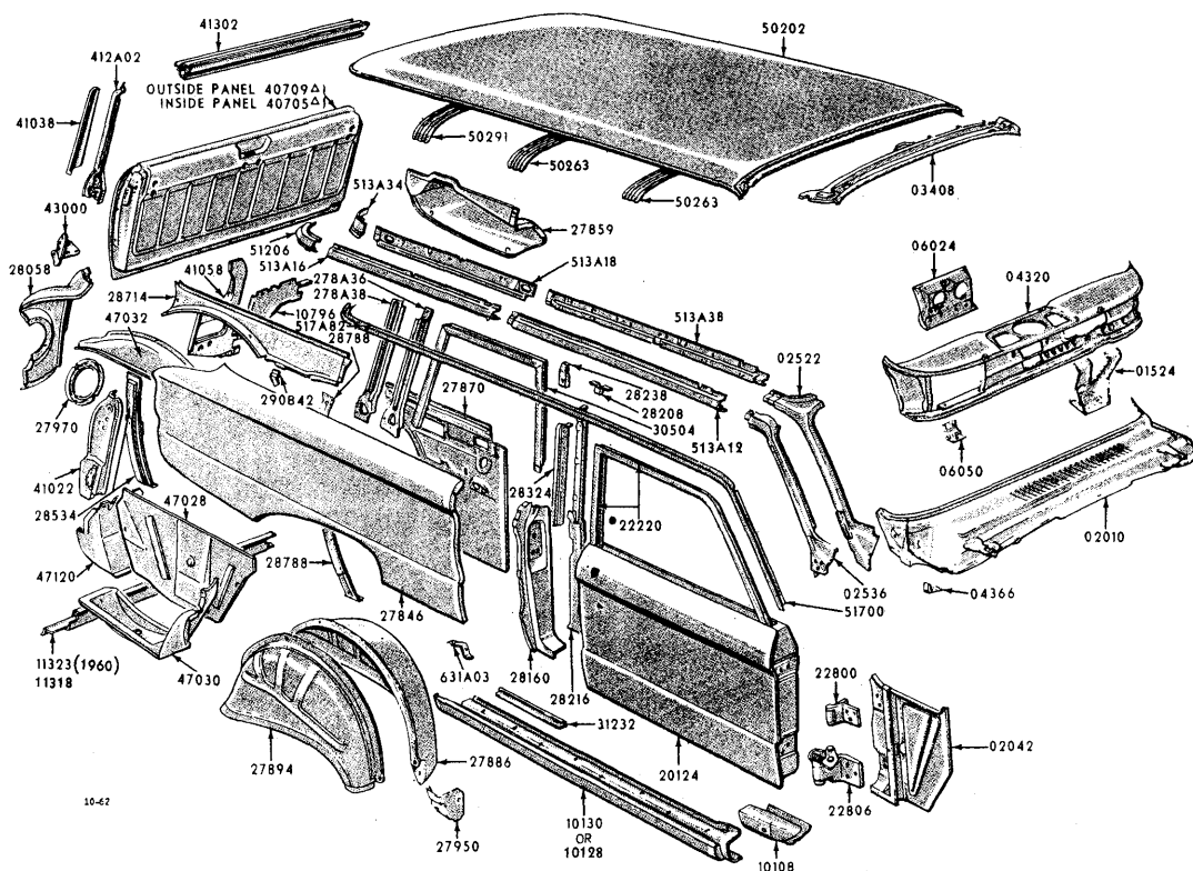
1960-61 FALCON RANCH WAGON AND SEDAN DELIVERY UPPER BODY - BODY TYPES X (59A, 78A)
