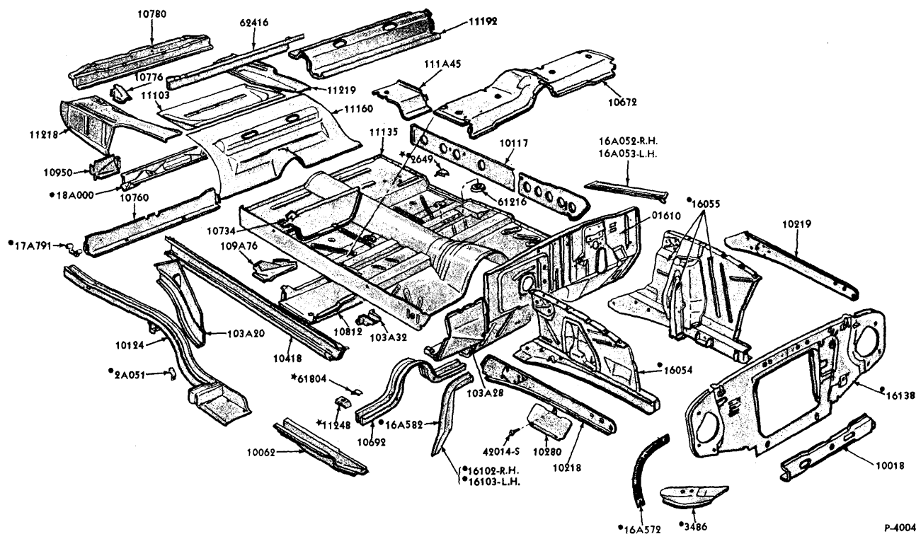
1963 FALCON CONVERTIBLE COUPE - UNDERBODY - BODY TYPE 76
