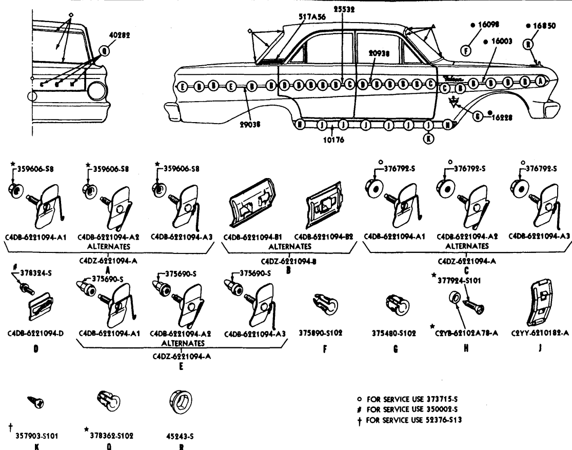
1964 FALCON TUDOR SEDAN - BODY TYPE X (62D)
