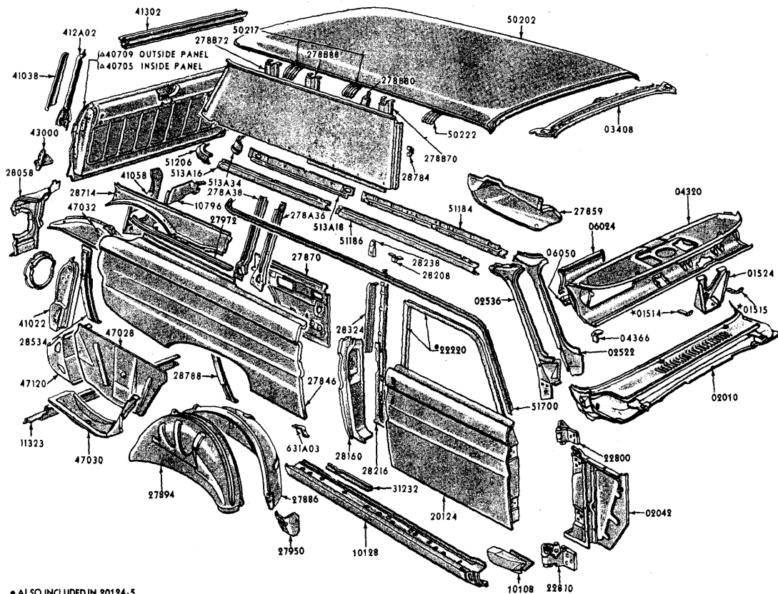
1964 FALCON SEDAN DELIVERY - UPPER BODY - BODY TYPE X (78)
