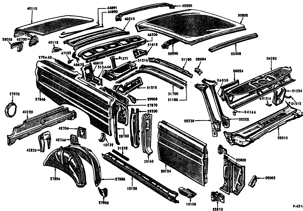
1964 FALCON "FUTURA" HARDTOP - UPPER BODY - BODY TYPE X (63)
