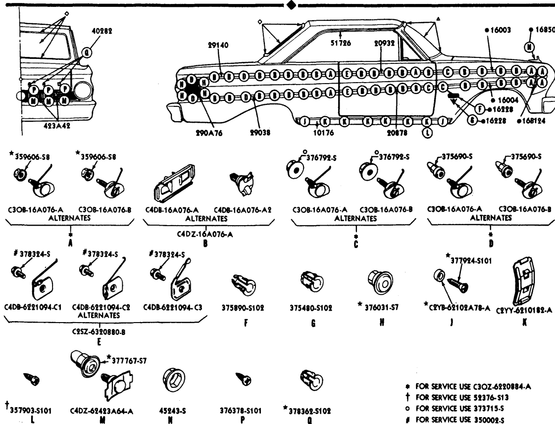
1964 FALCON "FUTURA" HARDTOP - BODY TYPES X (63B, 63C)
