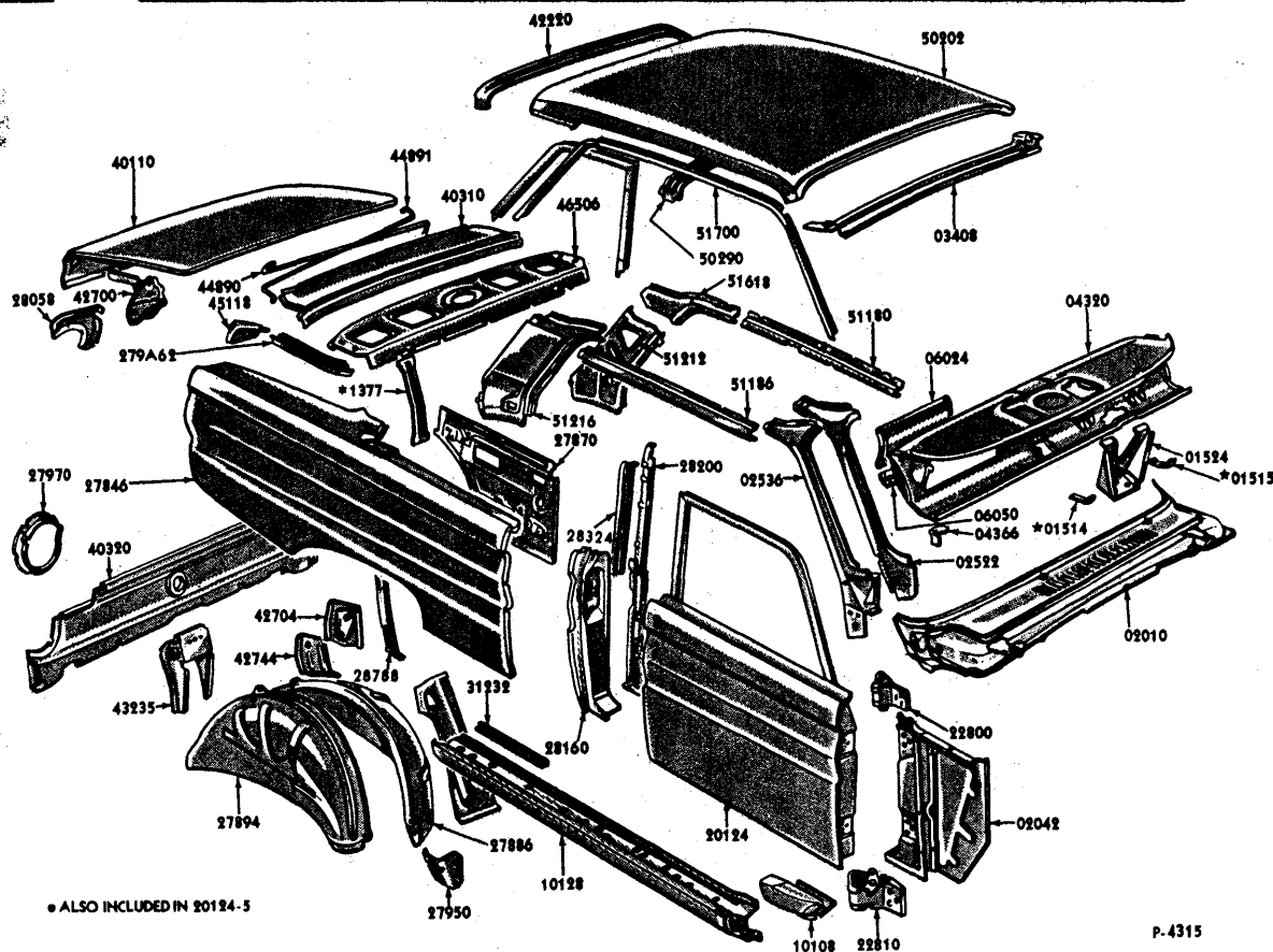
1964 FALCON TUDOR - UPPER BODY - BODY TYPE X (62)
