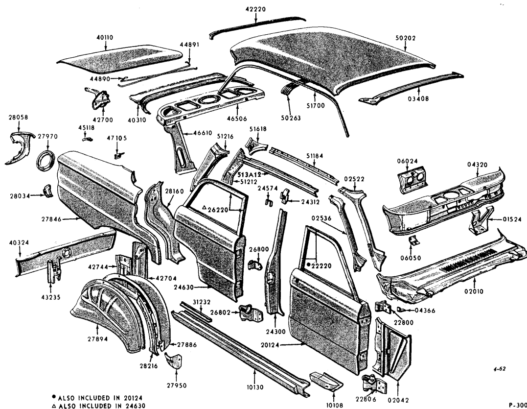
1960-62 FALCON FORDOR SEDAN - UPPER BODY - BODY TYPE 58A
