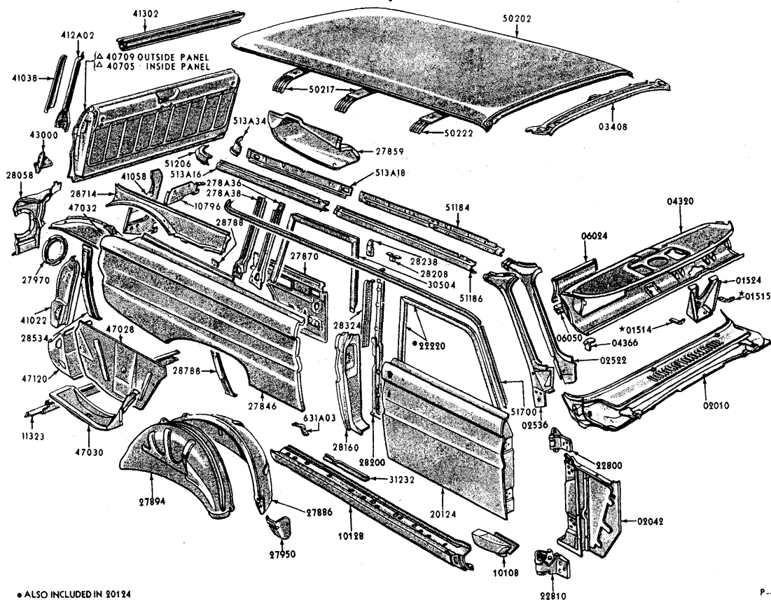
1964 FALCON TUDOR STATION WAGON - UPPER BODY - BODY TYPE X (59A)
