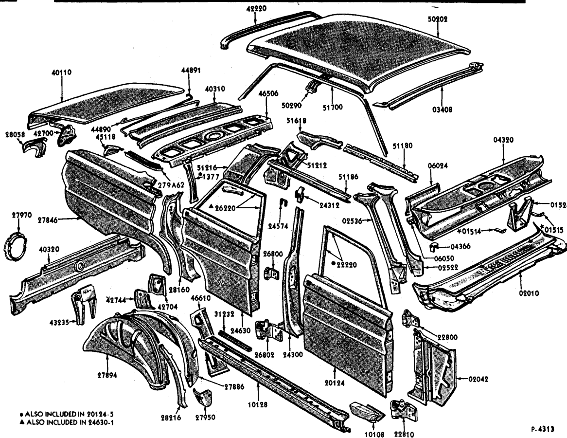
1964 FALCON FORDOR - UPPER BODY - BODY TYPE X (54)
