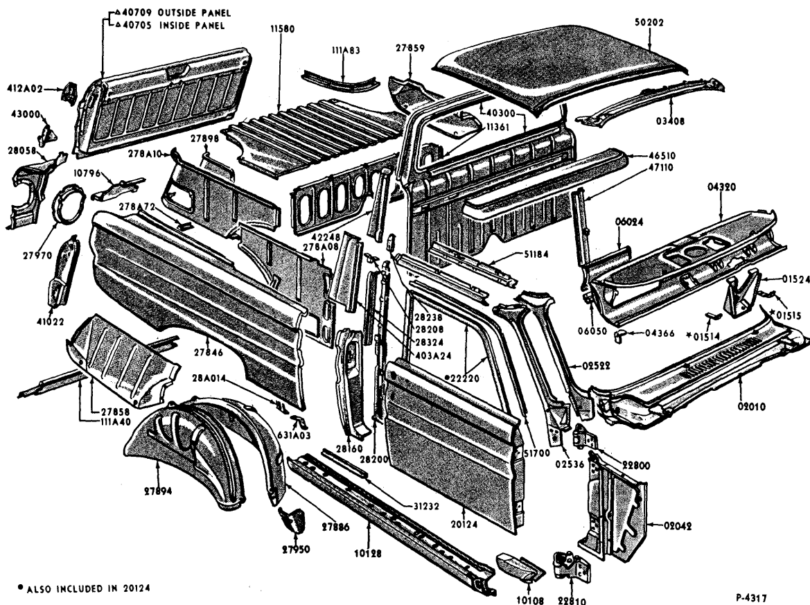
1964 FALCON "RANCHERO" - UPPER BODY - BODY TYPE X (66)
