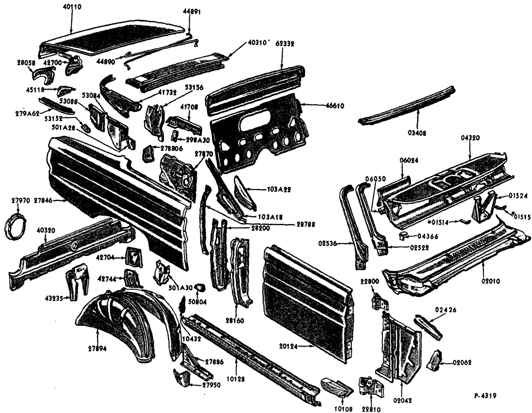
1964 FALCON CONV. COUPE - UPPER BODY - BODY TYPE X(76)
