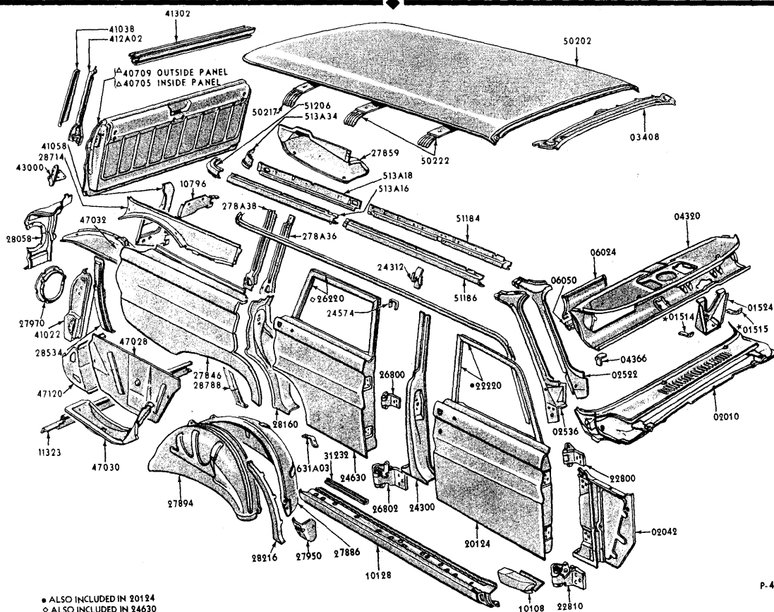
1964 FALCON FORDOR STATION WAGON - UPPER BODY - BODY TYPE X (71)
