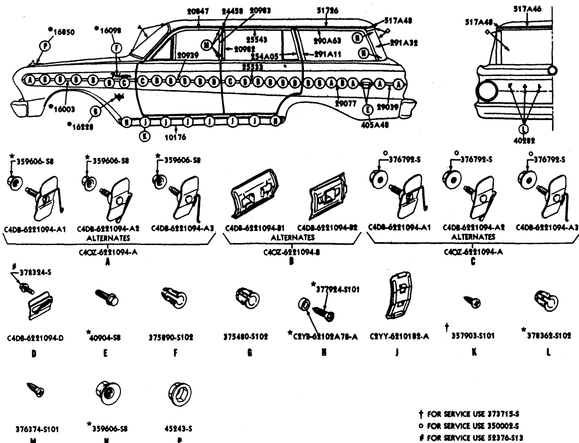
1964 FALCON FORDOR STATION WAGON - BODY TYPE X (71B)
