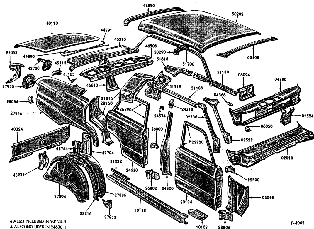
1963 FALCON FORDOR - UPPER BODY - BODY TYPE 54
