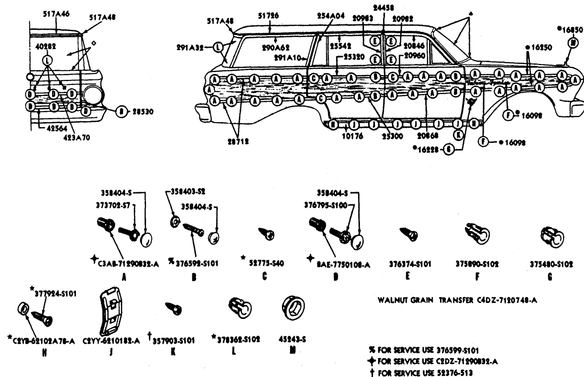
1964 FALCON FORDOR STATION WAGON - "COUNTRY SQUIRE" - BODY TYPE X (71C)
