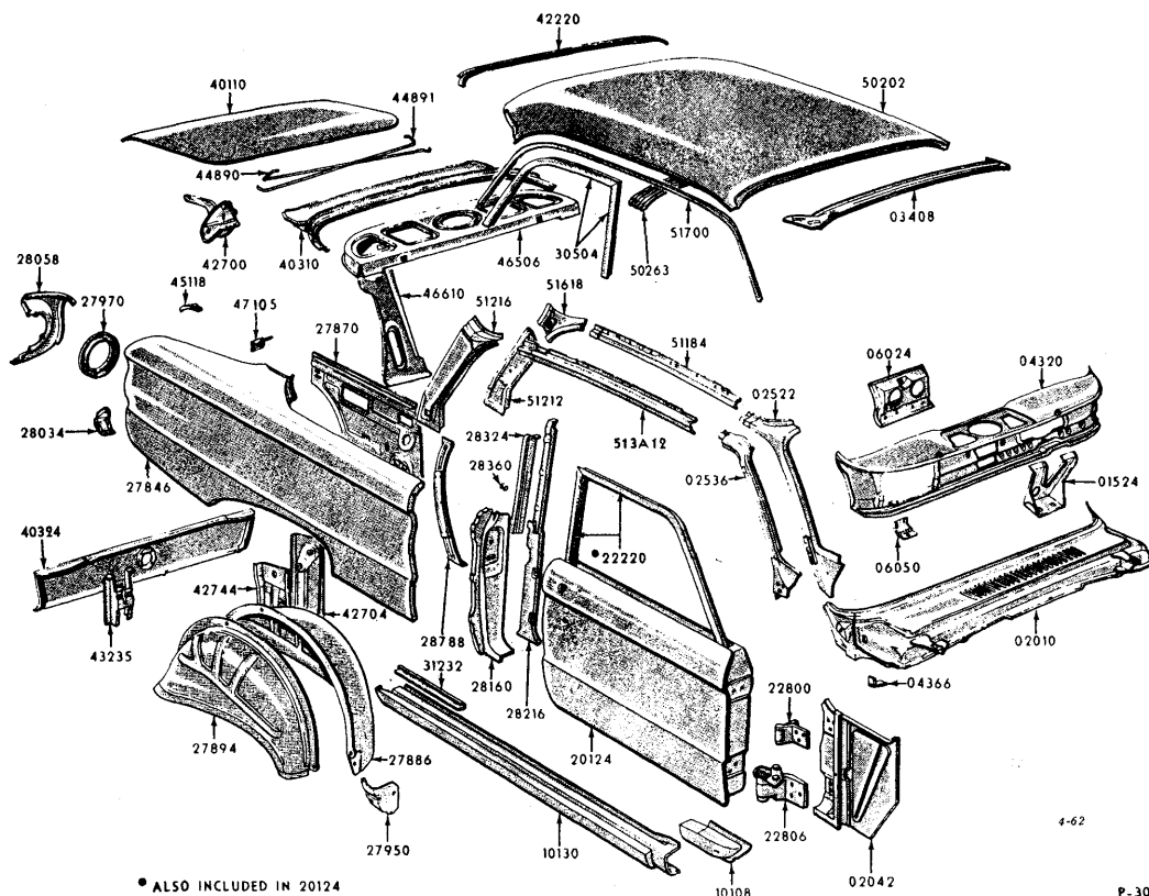
1960-61 FALCON TUDOR SEDAN UPPER BODY - BODY TYPE X (64)
